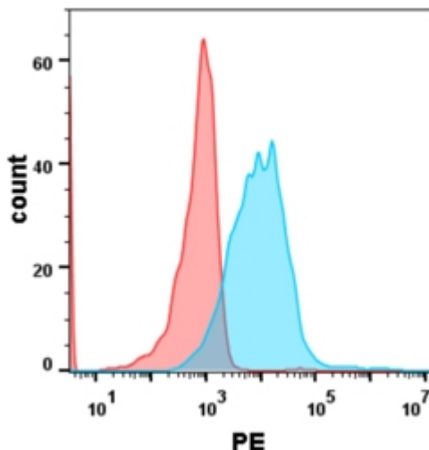
Figure 1. Flow cytometry analysis with Anti-GPRC5D mAb 25 \mu\text{g}/\text{ml} (Talquetamab) on Expi293 cells transfected with human GPRC5D (Blue histogram) or Expi293 transfected with irrelevant protein (Red histogram).
